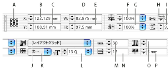
A Reference point B X Location C Y Location D Width E Height F Vertical scaling G Horizontal scaling H Character aki I Line aki J Grid format name K Grid view L Font size M Frame grid characters per line N Number of lines O Number of columns P Column gutter
